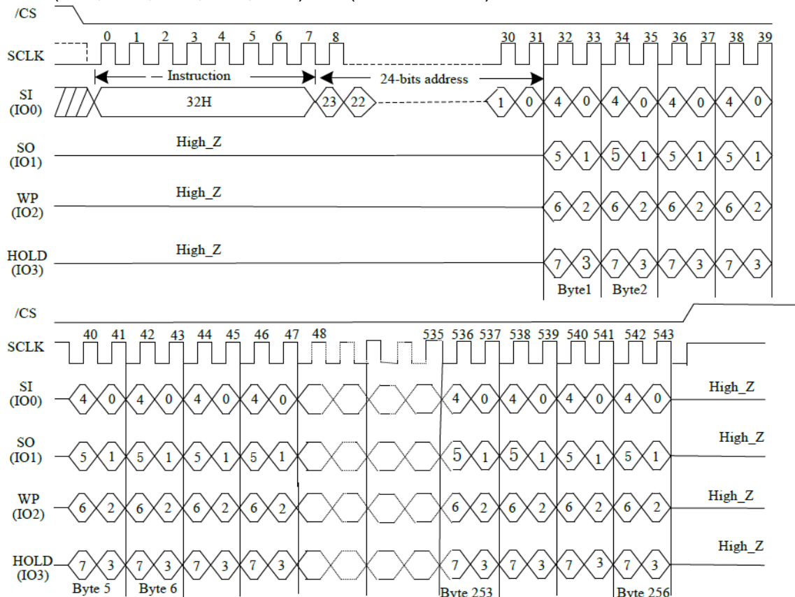
Figure 32. Qual Page Program Sequence Diagram
